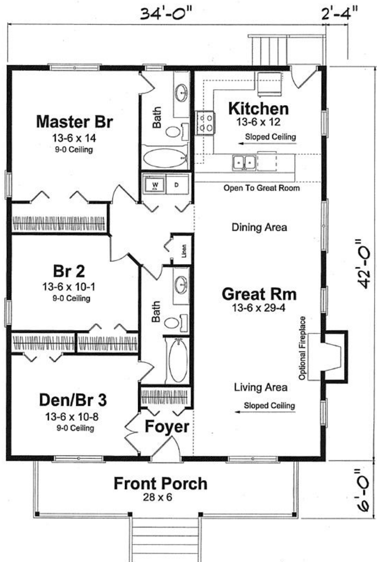
Floor Plan
